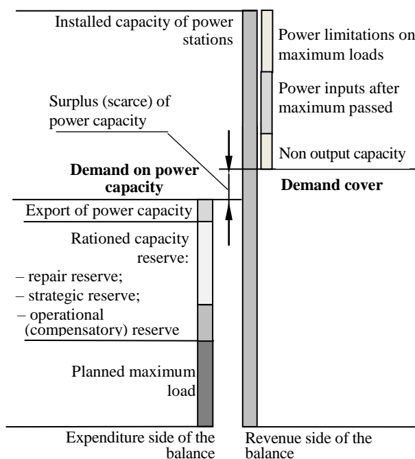
Fig. 1. Structure of the projected power balance.
